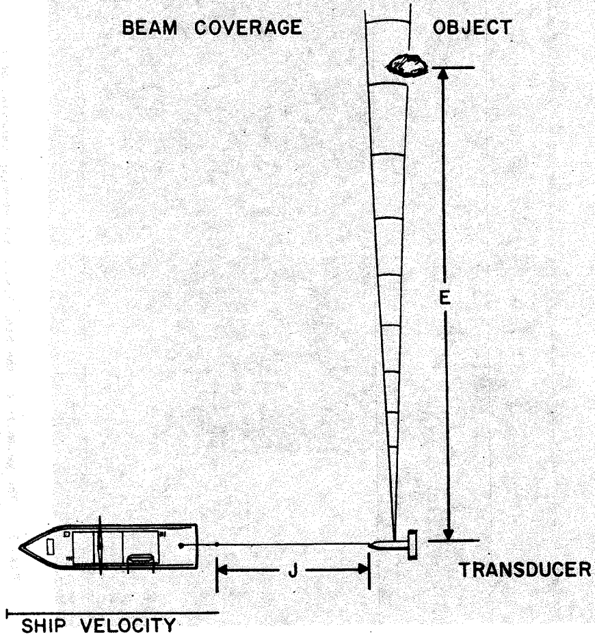
Fig. 1. Beam coverage of the Side Scan Sonar in the Horizontal plane.
