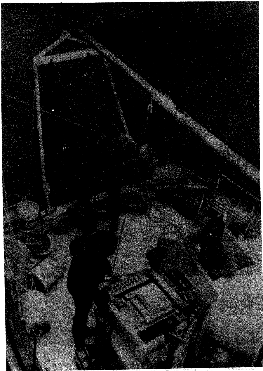
Photo 2. A typical Side Scan Sonar installed on a small survey boat.
